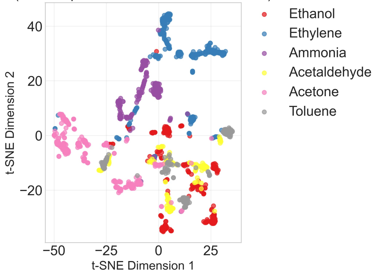
Latent Space by Gas Class (Good separation = effective classification)
