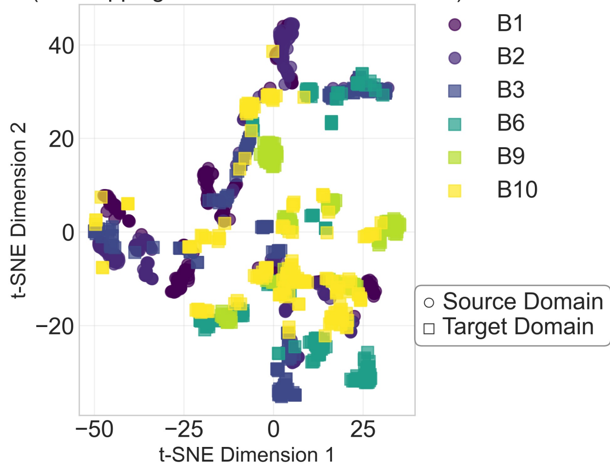
Latent Space by Batch (Overlapping = domain-invariant features)
